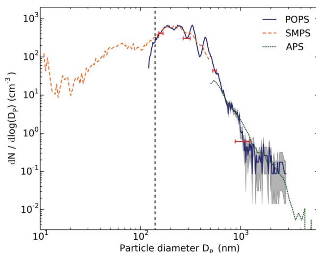
Figure 10. Intercomparison of POPS, SMPS, and APS. All three instruments were sampling air pulled from a 12.5-m inlet. The data shown were 10-min averages. Vertical dashed line indicates the POPS lower detection limit with 100% detection efficiency. Grey shading indicates the POPS counting uncertainty. Horizontal bars represent POPS sizing uncertainties.
