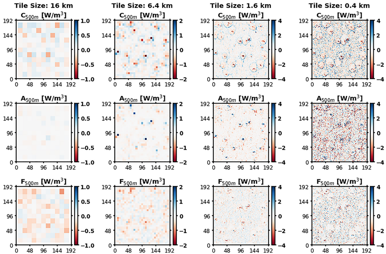
Figure B5. Snapshots of the (top) C , (middle) A , and (bottom) F terms at 500 m altitude from the Diel+12h simulation at hour 16. The terms are computed at various tile sizes: 16, 6.4, 1.6, and 0.4 km. Note the different scales of the color bars for different tile sizes.
