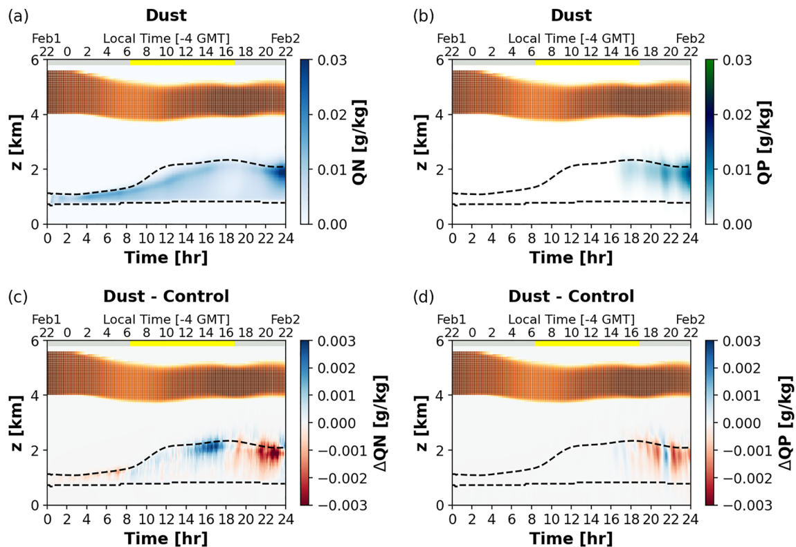
Figure 9. Domain-mean time series of (a, b) cloud and rain water mixing ratios (QN and QP, respectively) from the Dust simulation. (c, d) Differences in QN and QP between the Dust and Control simulations. The black dashed lines indicate the cloud top and base heights of the Dust simulation. The brown shading indicates the mineral-dust layer. The bottom x-axes indicate the time after the simulations begin and the top x-axes indicate the local time of the simulations, as in Figure 2.
