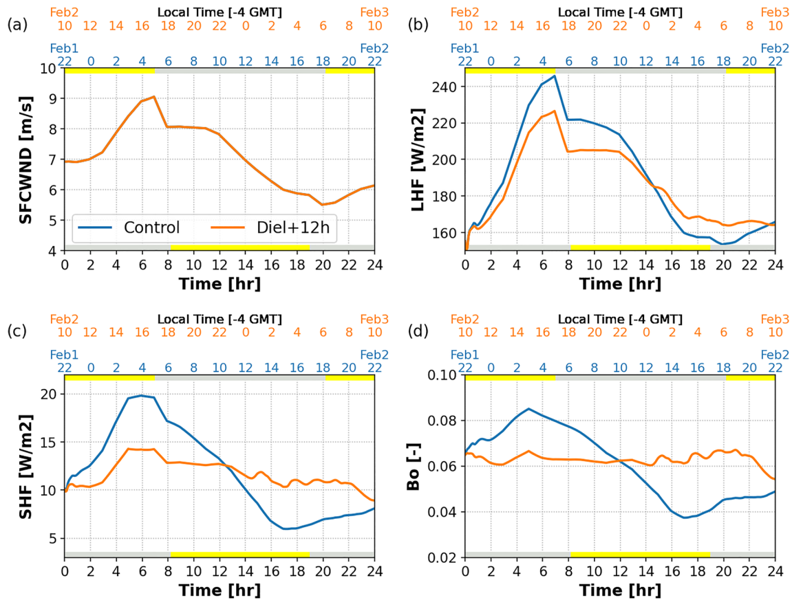
Figure A1. As in Figure 1 but for (a) the surface wind speed, (b) the surface latent heat flux (LHF), (c) surface sensible heat flux (SHF), and (d) the Bowen ratio ( Bo = SHF/LHF ) from the Control and Diel+12h simulations.
